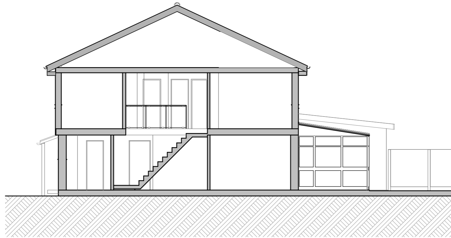
Building Section
