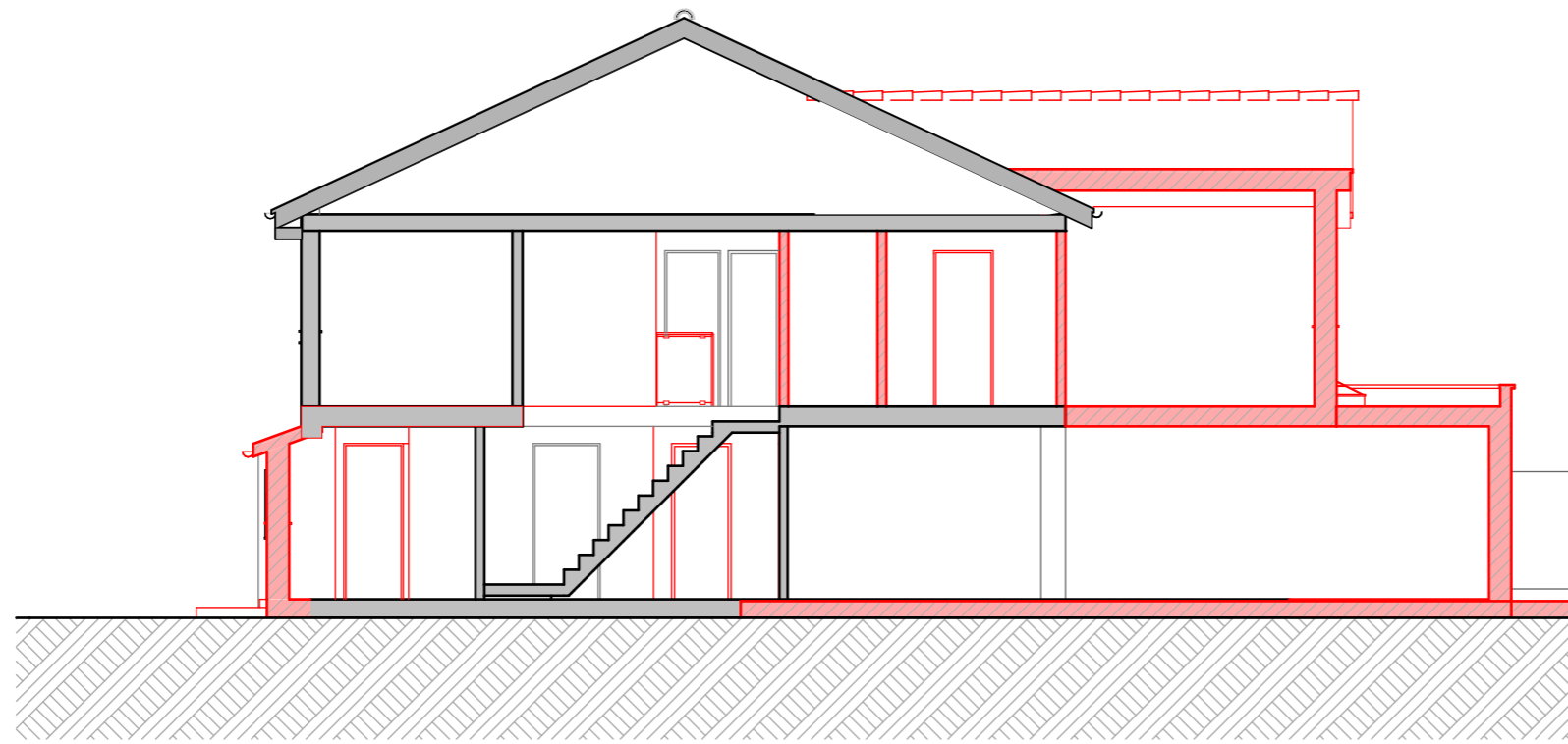
Building Section
