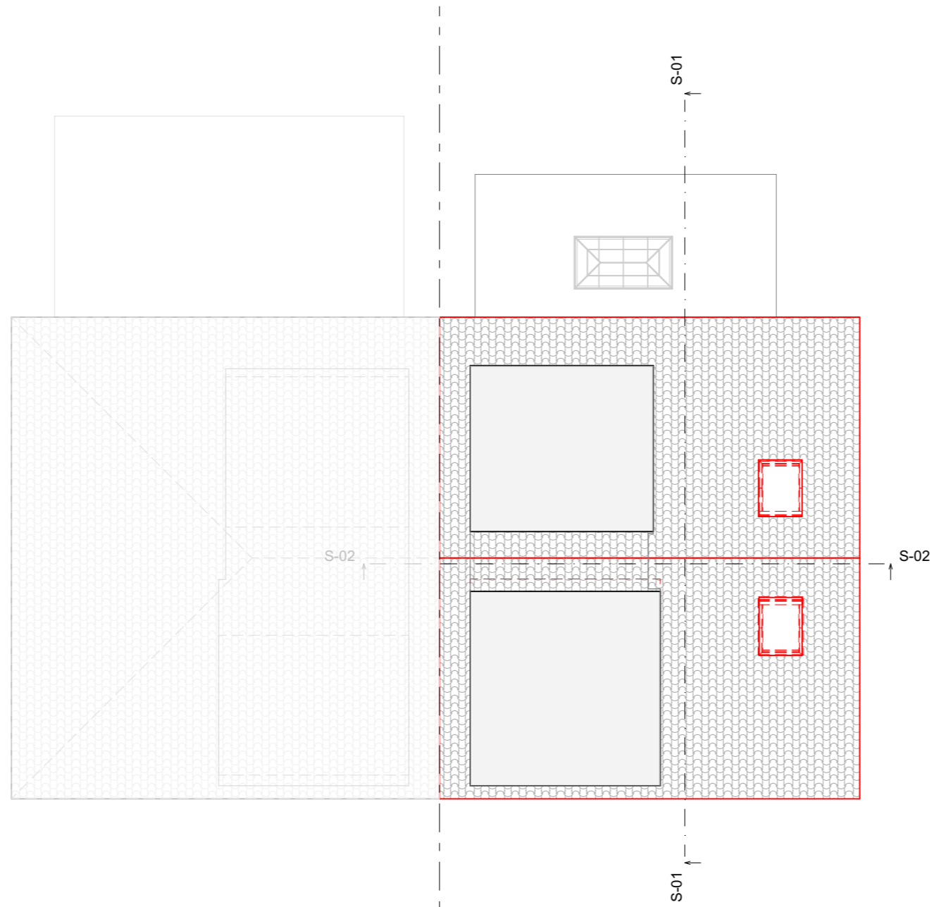
Roof Plan
