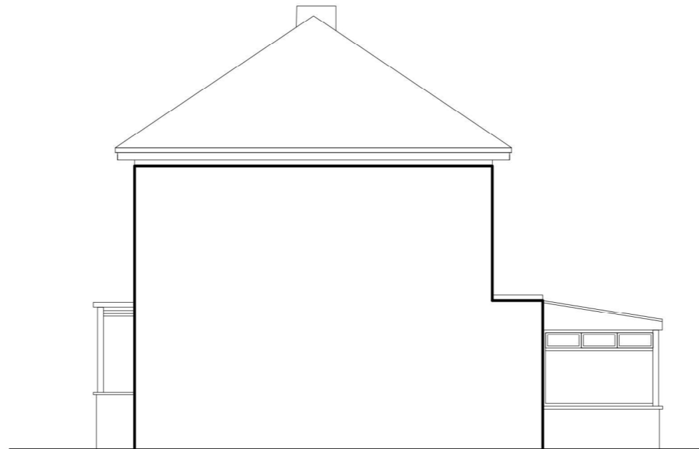
Existing West Elevation 1-100
