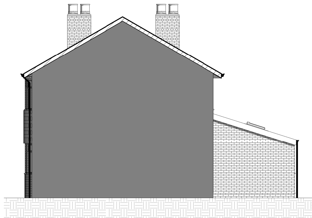
Right Elevation Proposed 1 : 100
