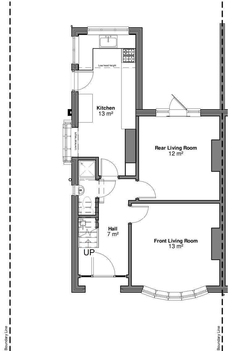
Ground Floor Existing 1 : 100
