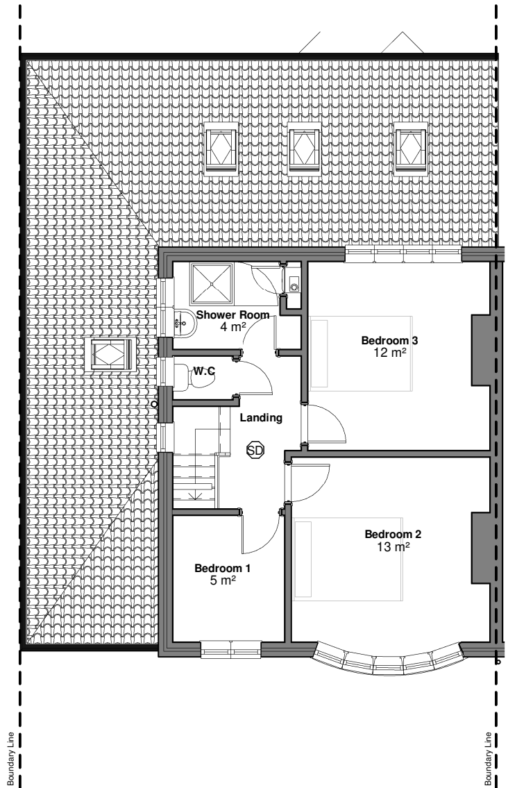
First Floor Proposed 1 : 100
