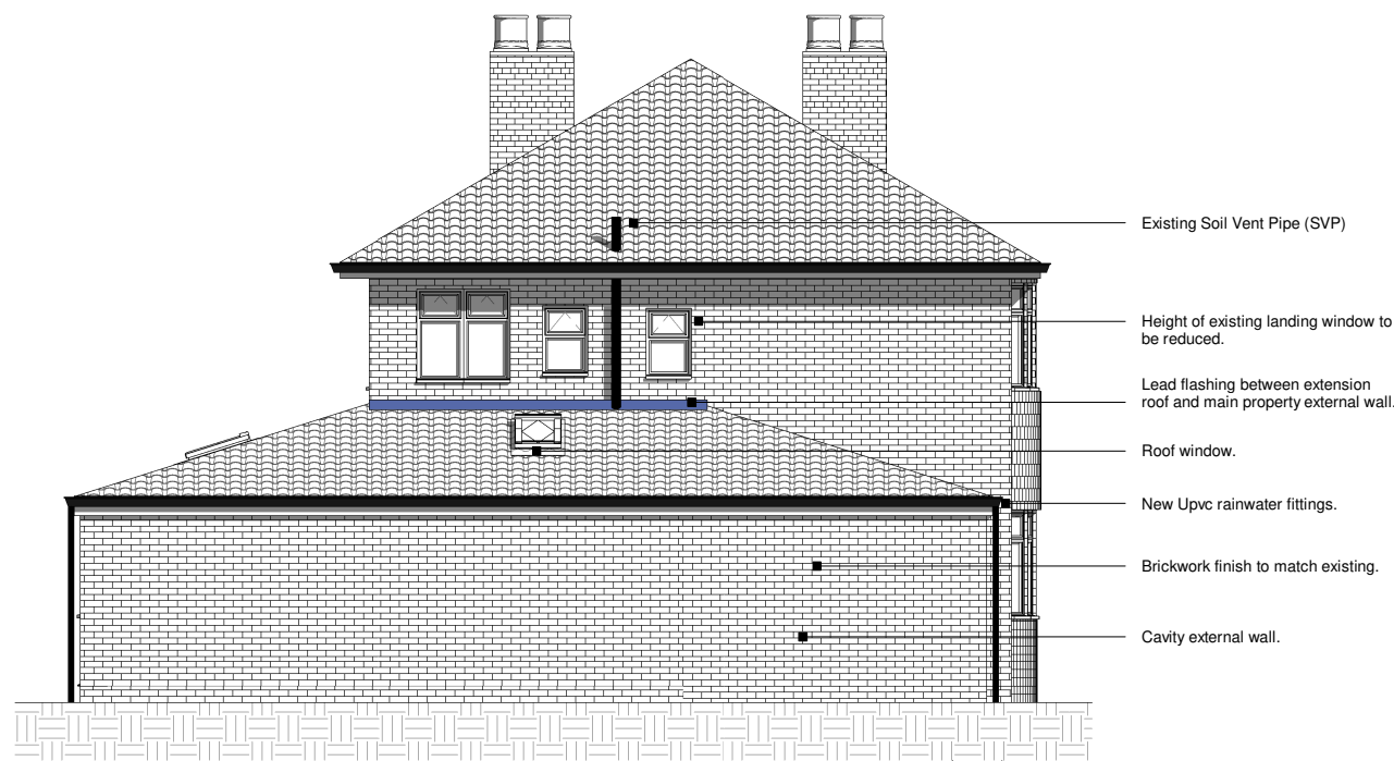
Left Elevation Proposed 1 : 100
