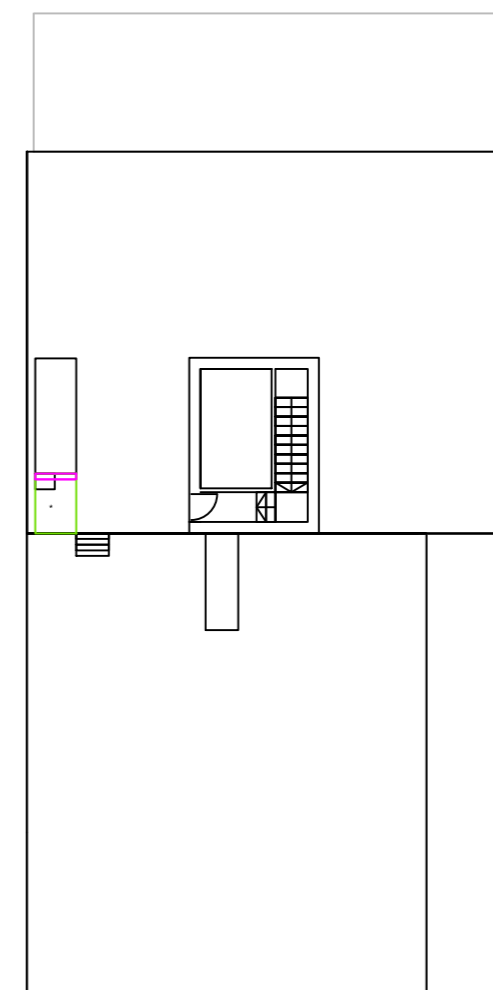
Roof Plan
