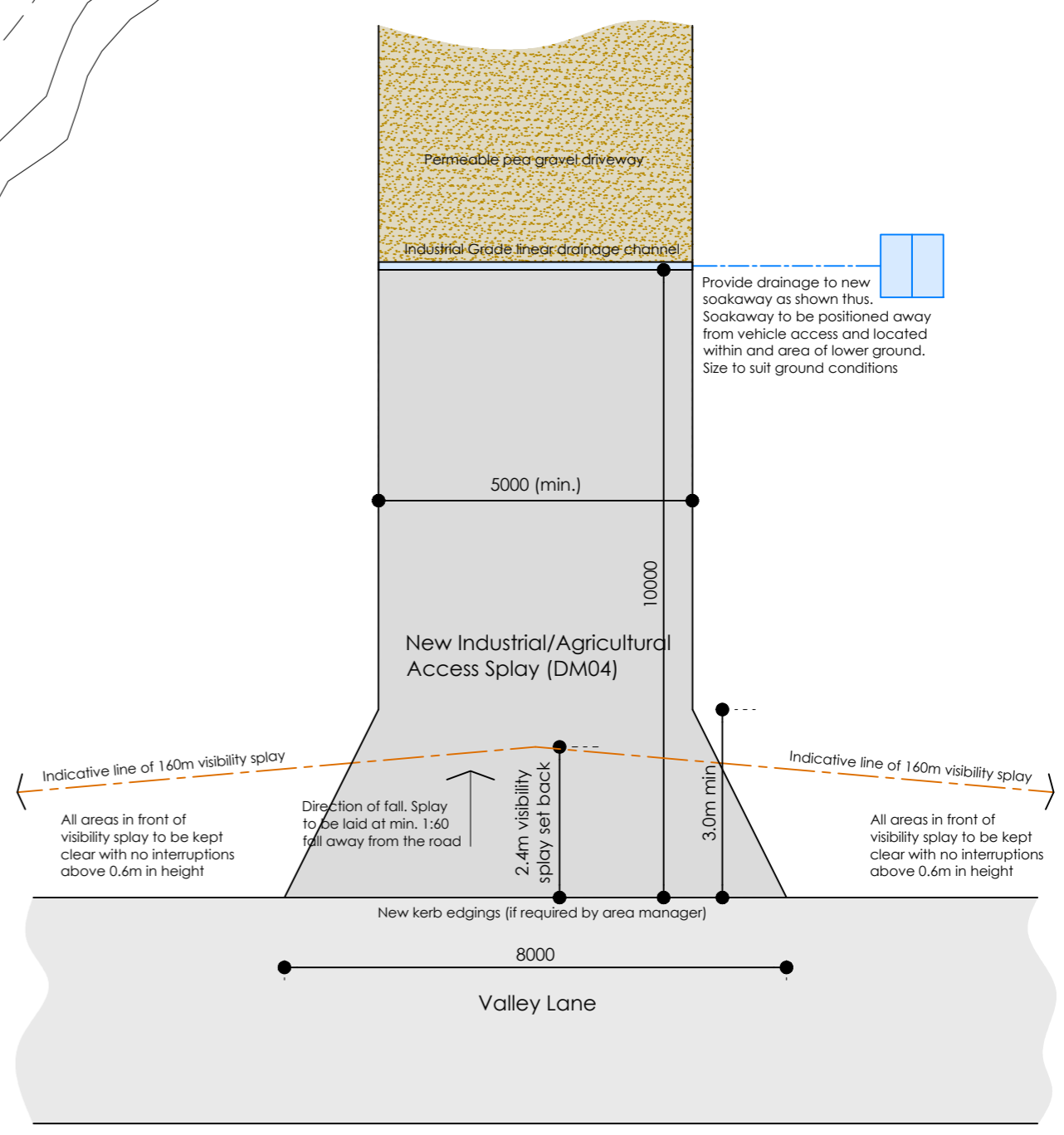
Access Splays Details 1:100
