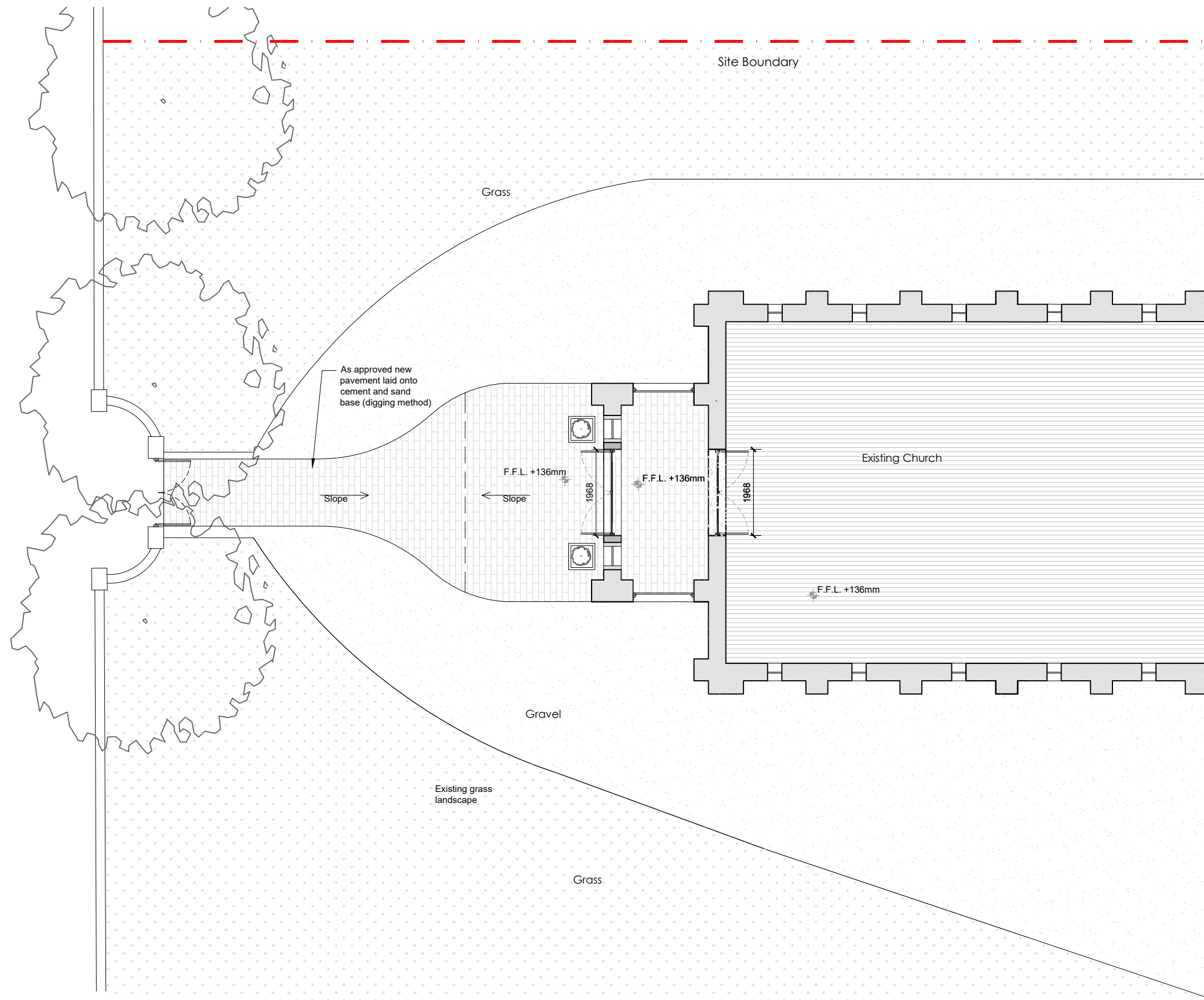
1 As Approved Landscape Plan 1:100
