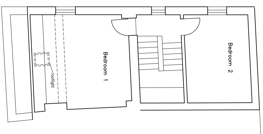
Second Floor
