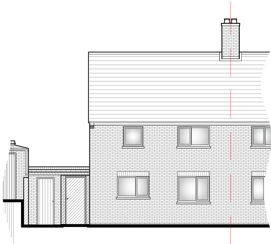
EXISTING WEST REAR ELEVATION
