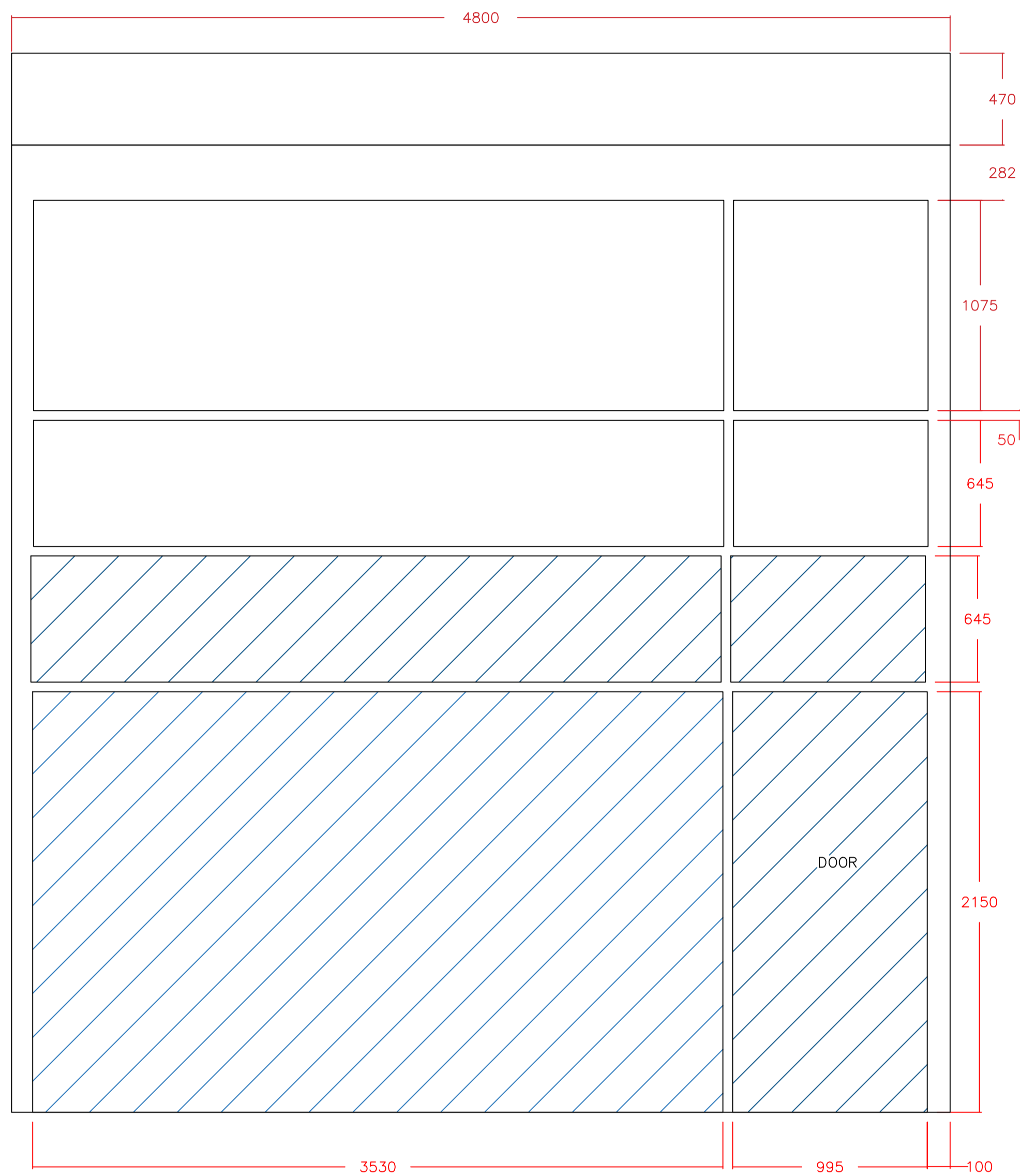
1 EXISTING ELEVATION - FRONT OF SHOP Scale: 1:20
