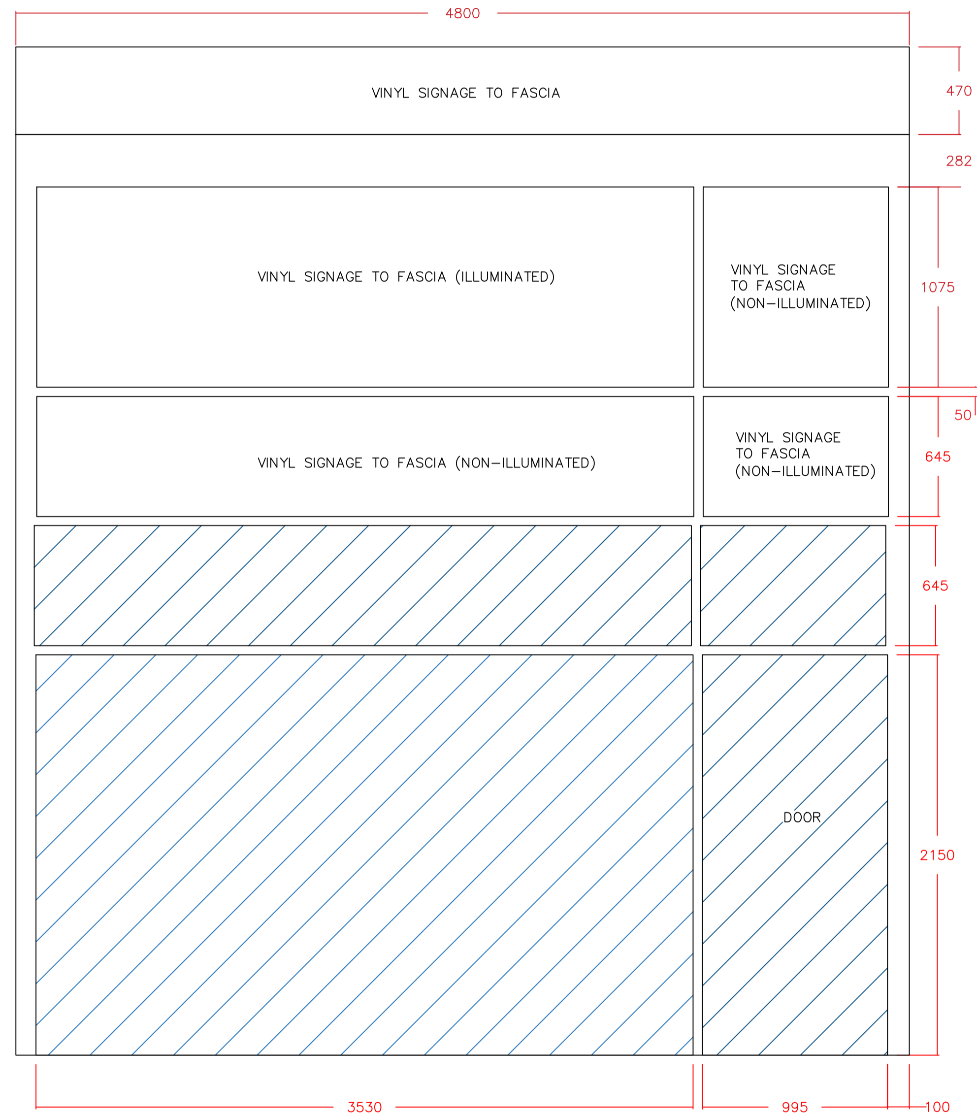
1 PROPOSED ELEVATION - FRONT OF SHOP Scale: 1:20
