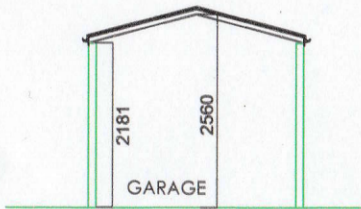
SECTION GARAGE
