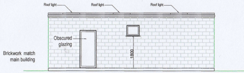
REAR ELEVATION
