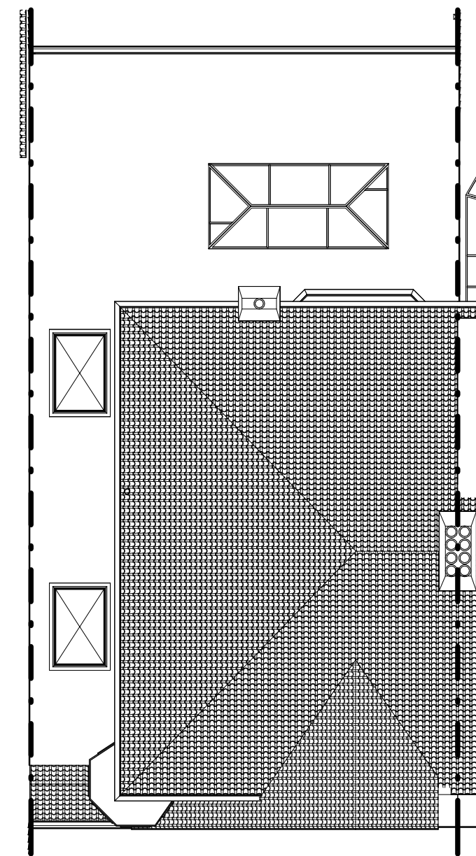
2 Proposed Roof Plan. 1 : 100
