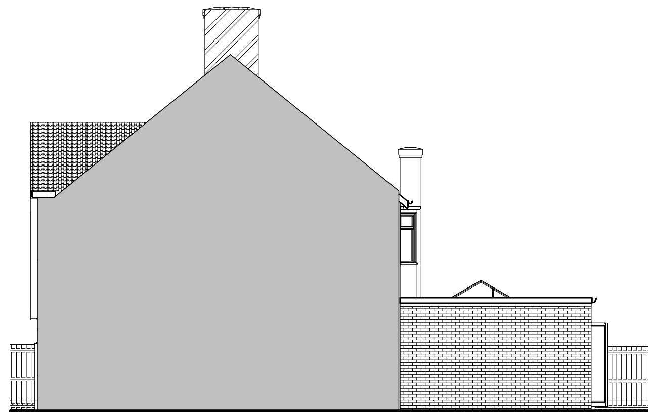
2 Proposed Side Elevation 1 : 100
