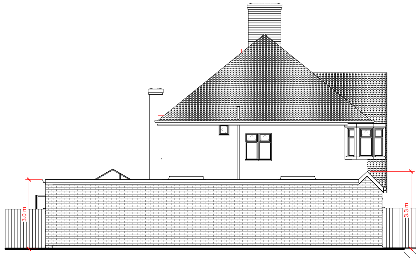
2 Proposed Side Elevation II 1 : 100
