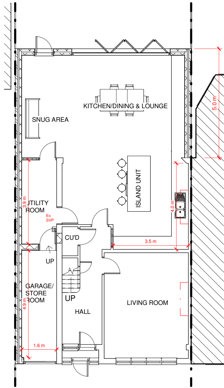
1 Proposed Ground Floor 1 : 100
