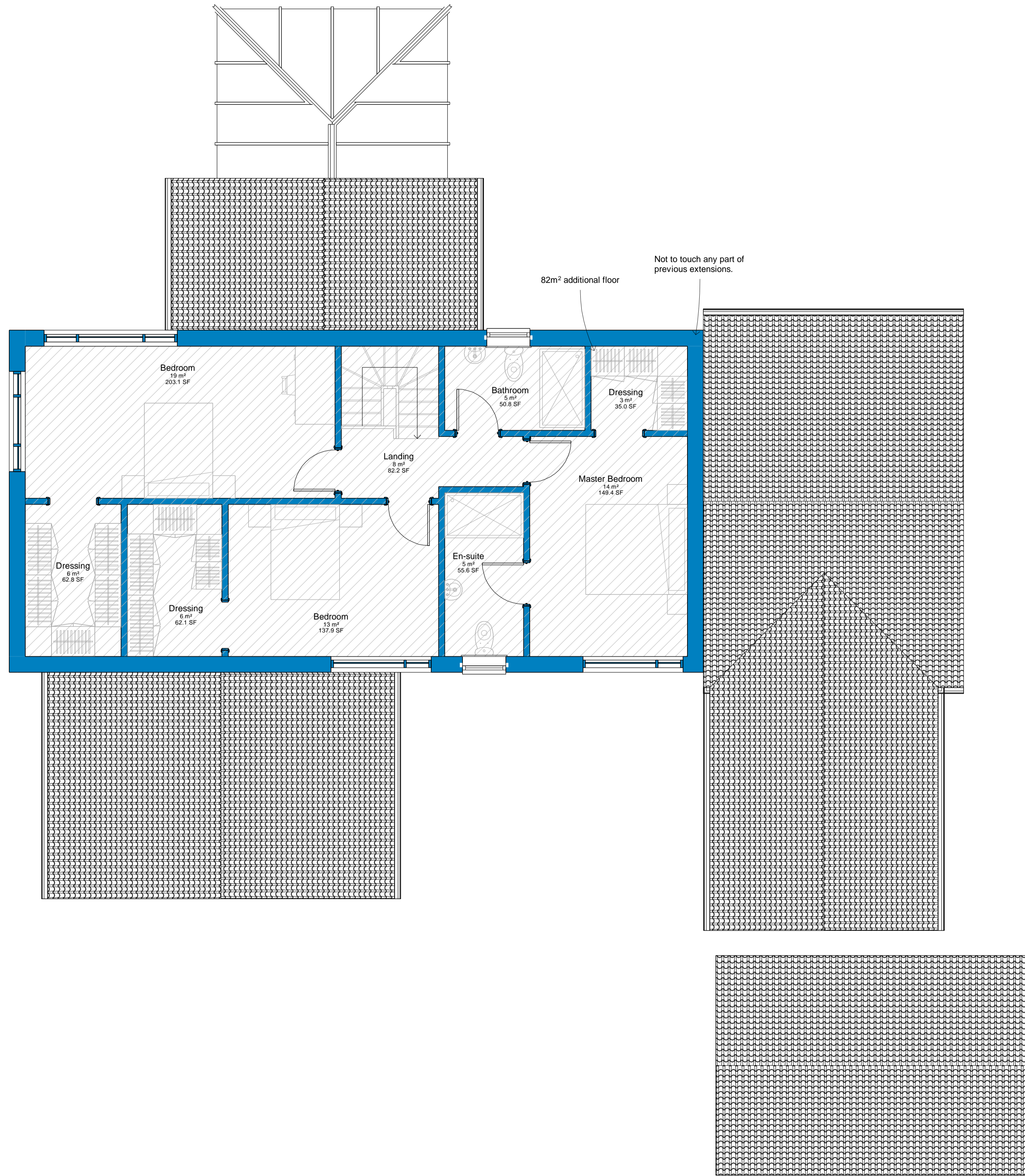
1 First Floor -As Proposed 1 : 50
