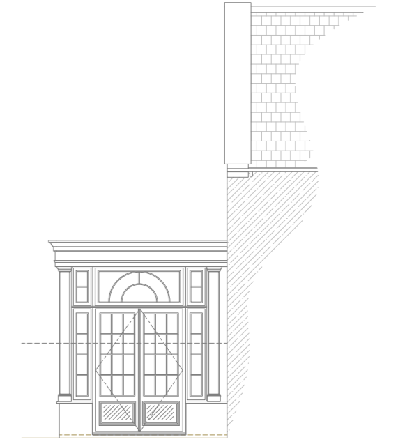
PROPOSED SIDE ELEVATION/SECTION Scale 1:100
