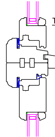
Window Head Rail
