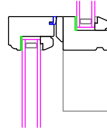
Sashes in Centre
