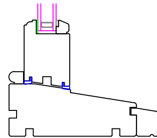
Window Bottom Rail
