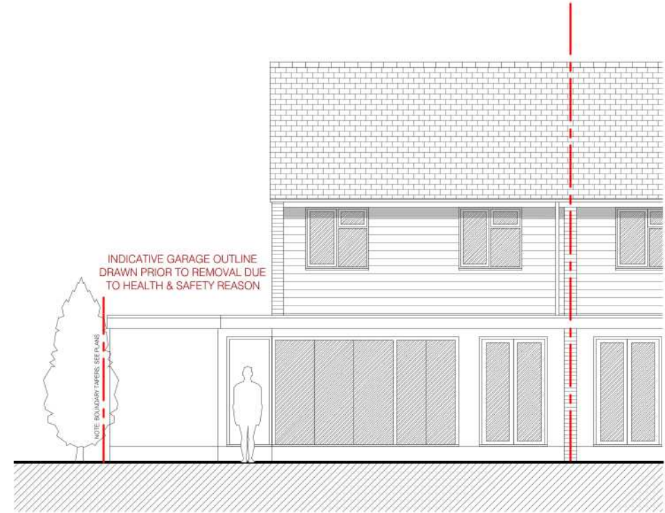
existing drawing REAR ELEVATION
