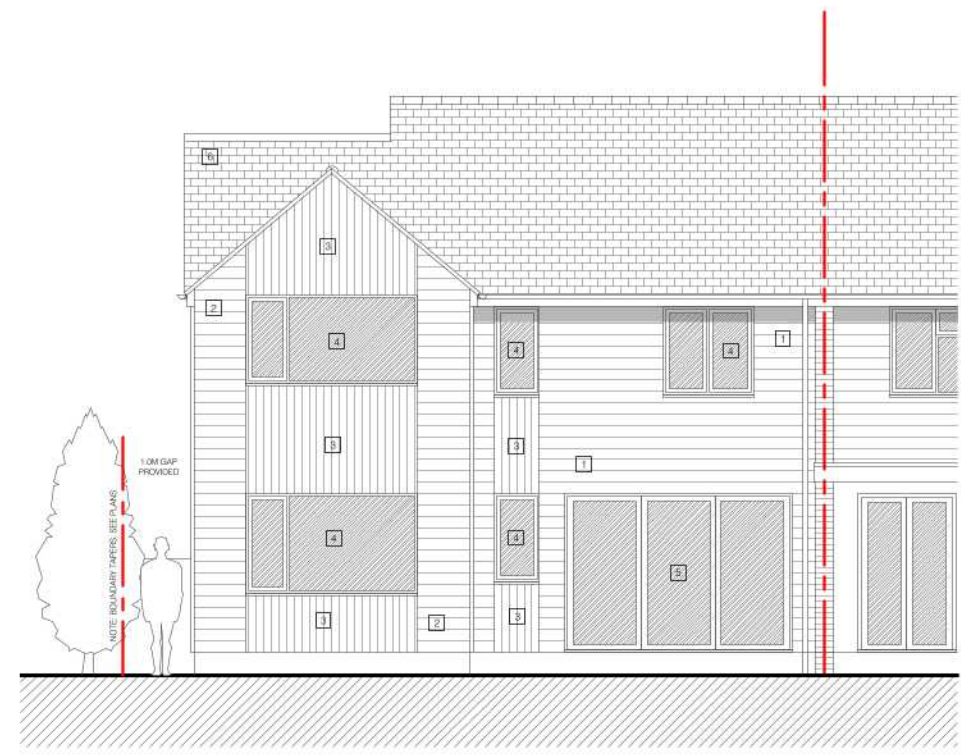
proposed drawing REAR ELEVATION
