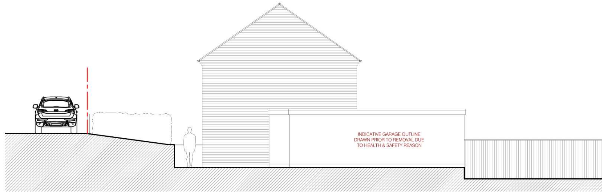
existing drawing SIDE ELEVATION
