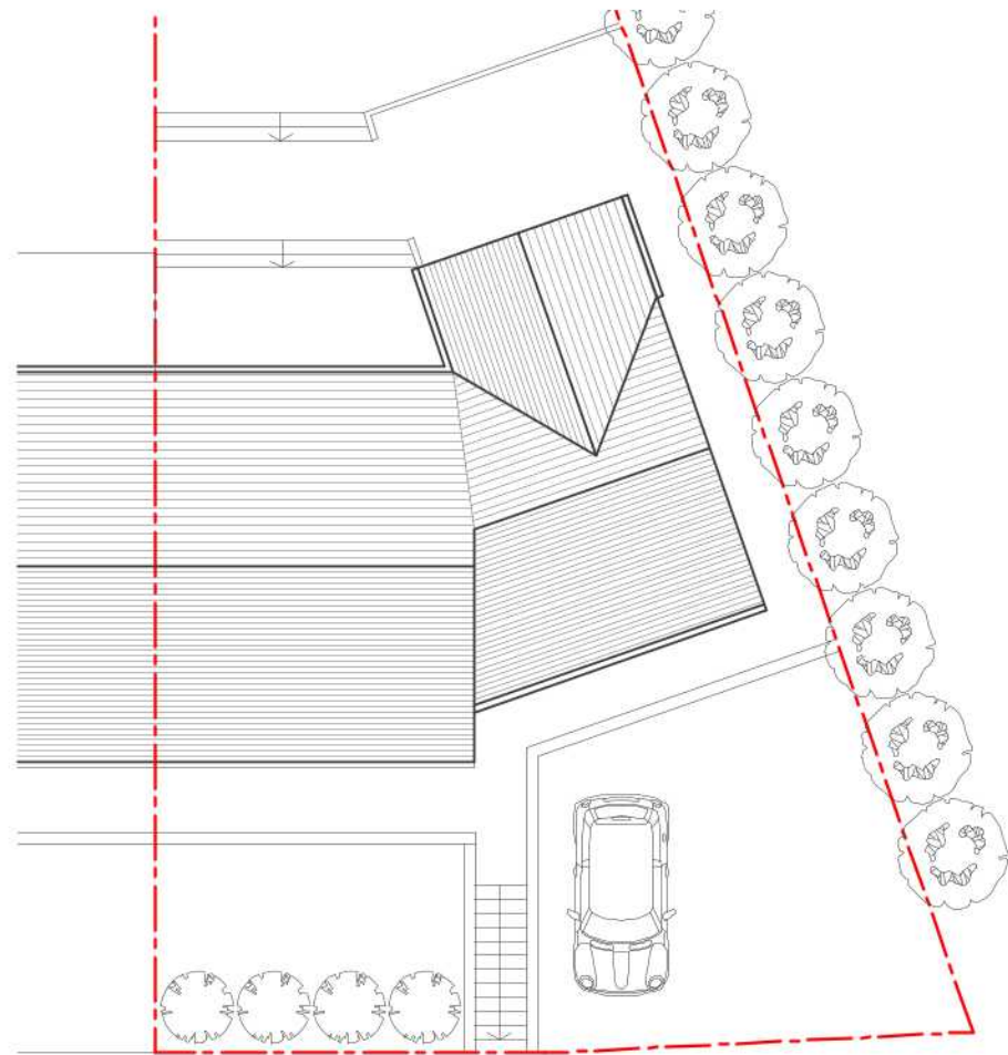
proposed drawing ROOF PLAN - NTS
