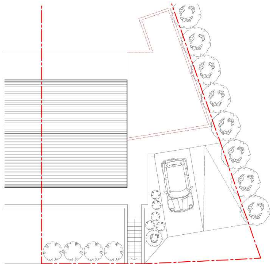
existing drawing ROOF PLAN - NTS
