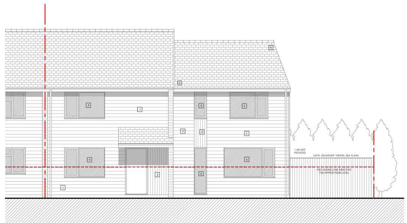
proposed drawing FRONT ELEVATION
