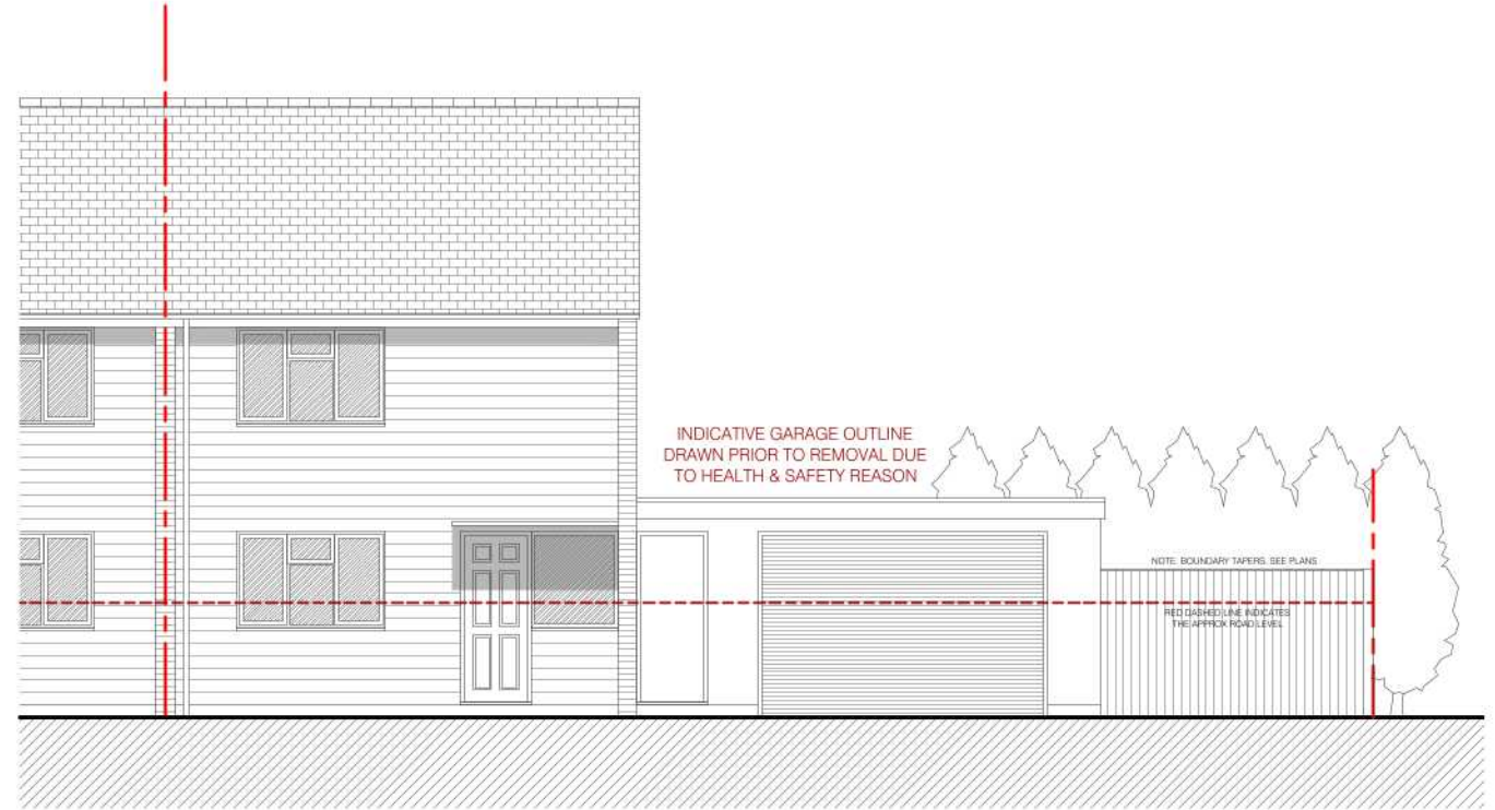
existing drawing FRONT ELEVATION
