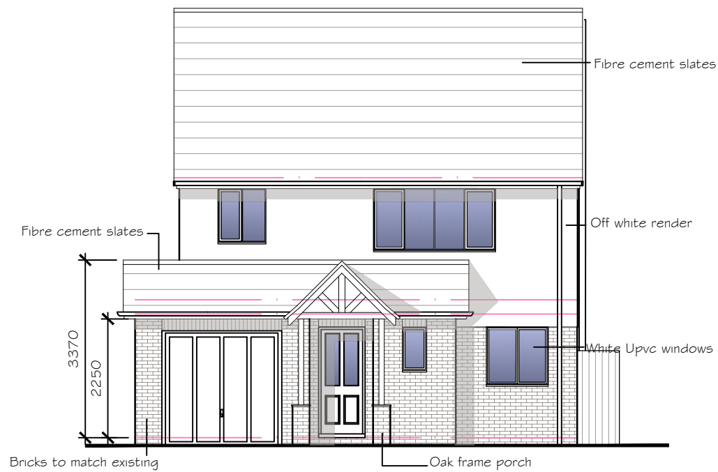
FRONT ELEVATION
