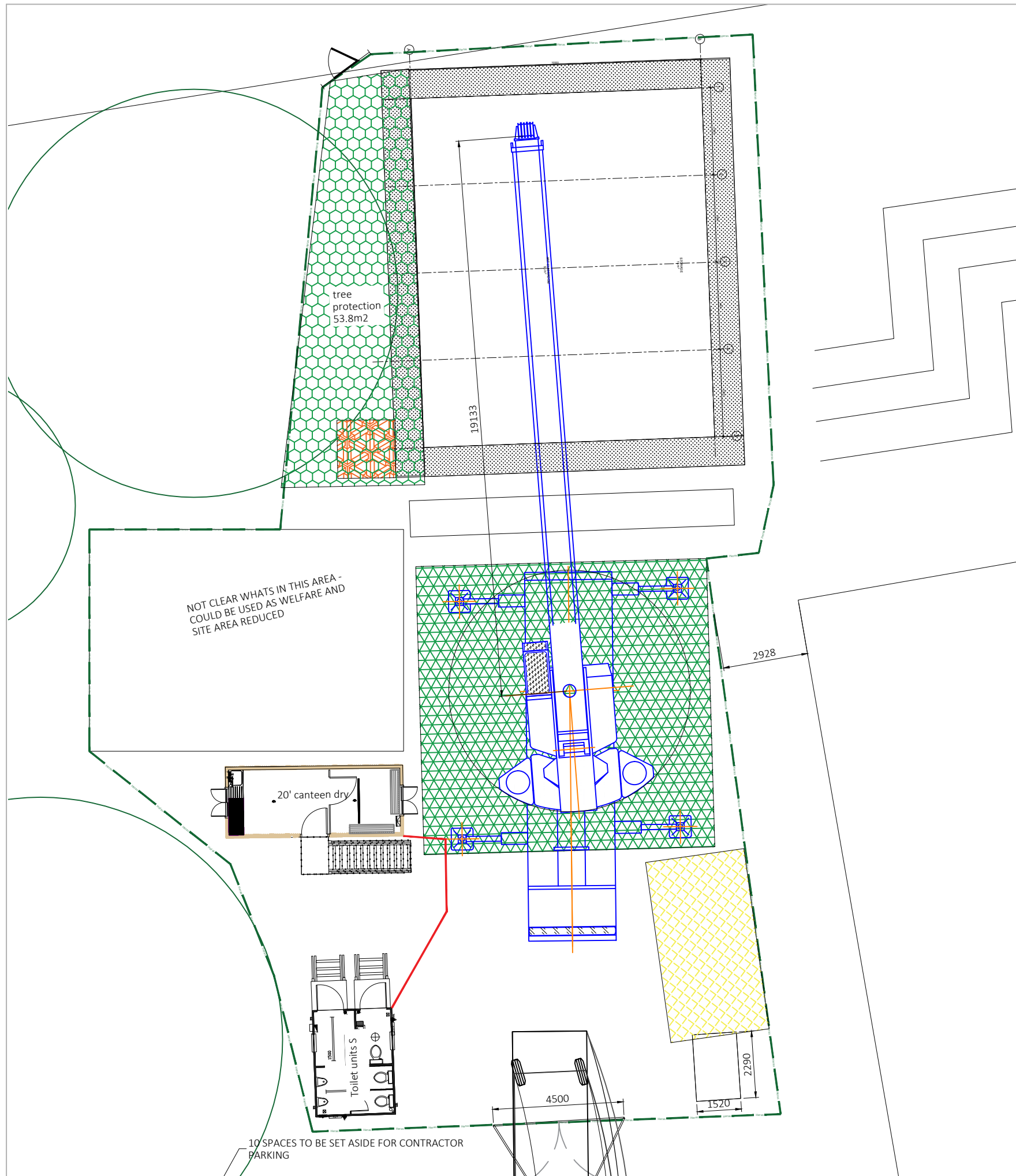
1:150 - Site compound Sheet Size: A3 © Modulek Ltd
