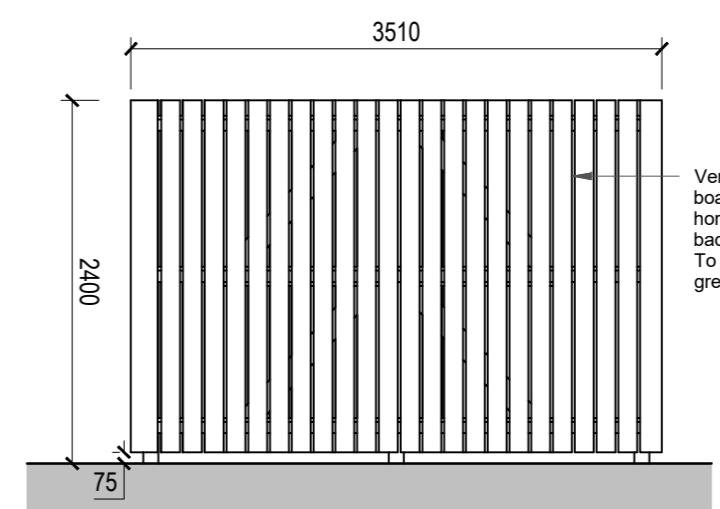
Rear Elevation Scale @ 1:50
