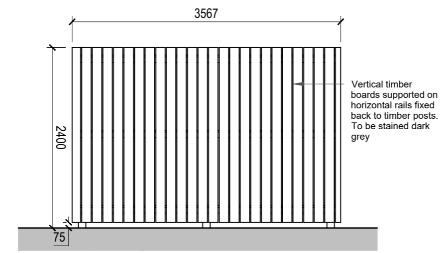
Short Elevation Scale @ 1:50
