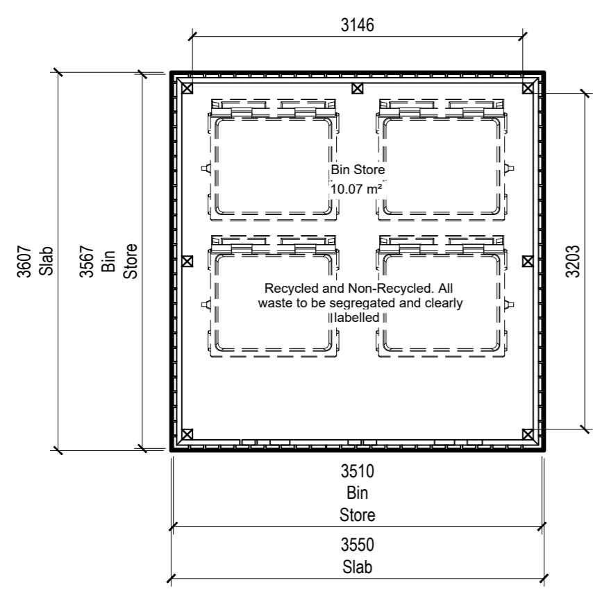
Bin Store Plan Scale @ 1:50
