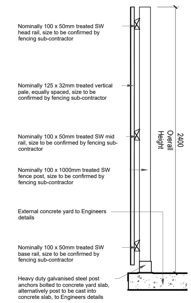
Bin Store Detail Section Scale @ 1:20
