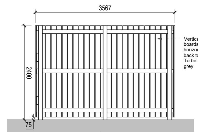
Bin Store Section Scale @ 1:50
