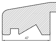
47MM CILL EXTENSION
