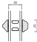
25MM BONDED BAR
