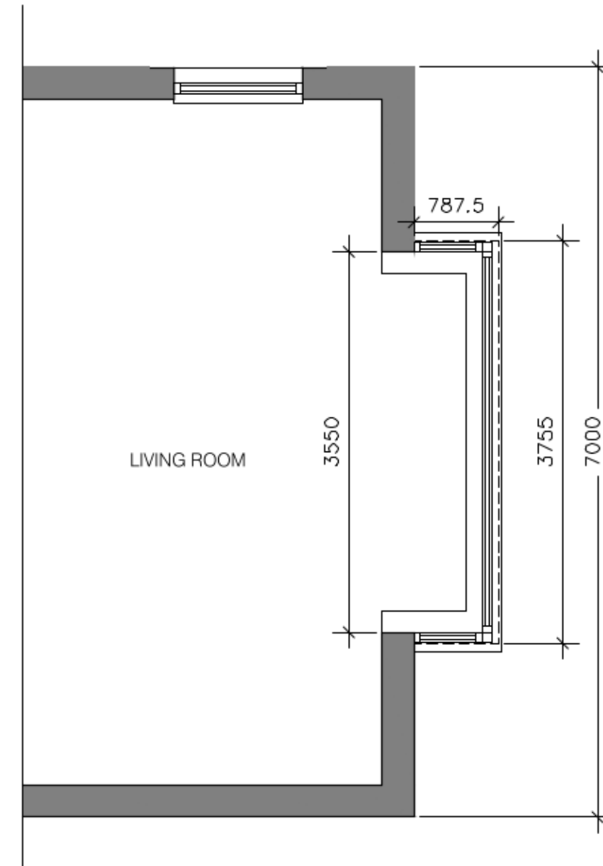
FLOOR PLAN ABOVE CILL 1:50
