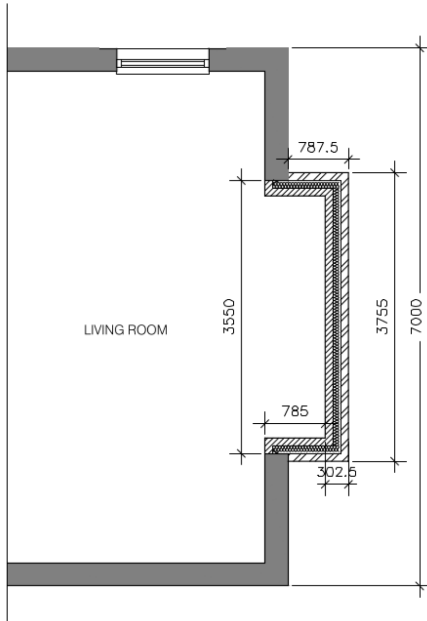
FLOOR PLAN BELOW CILL 1:50
