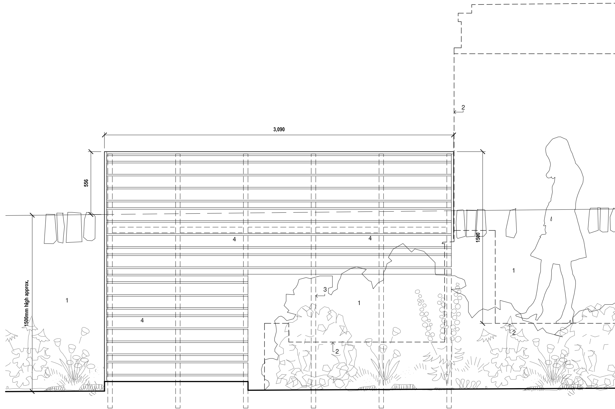
Screen elevation scale 1:20
