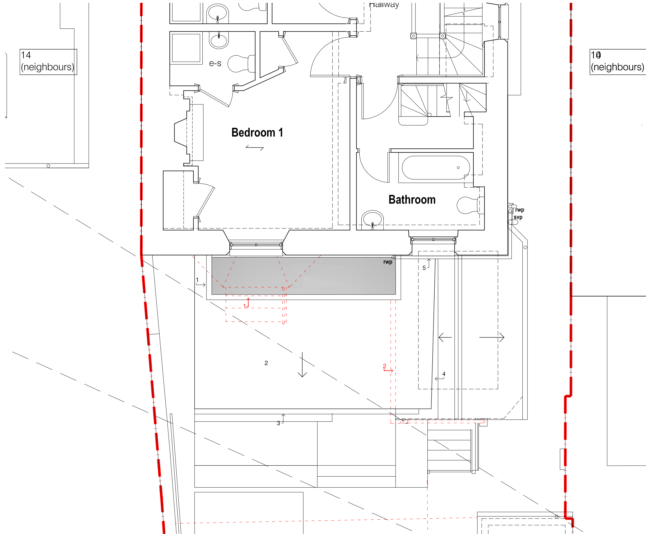
First Floor / Roof Plan scale 1:50
