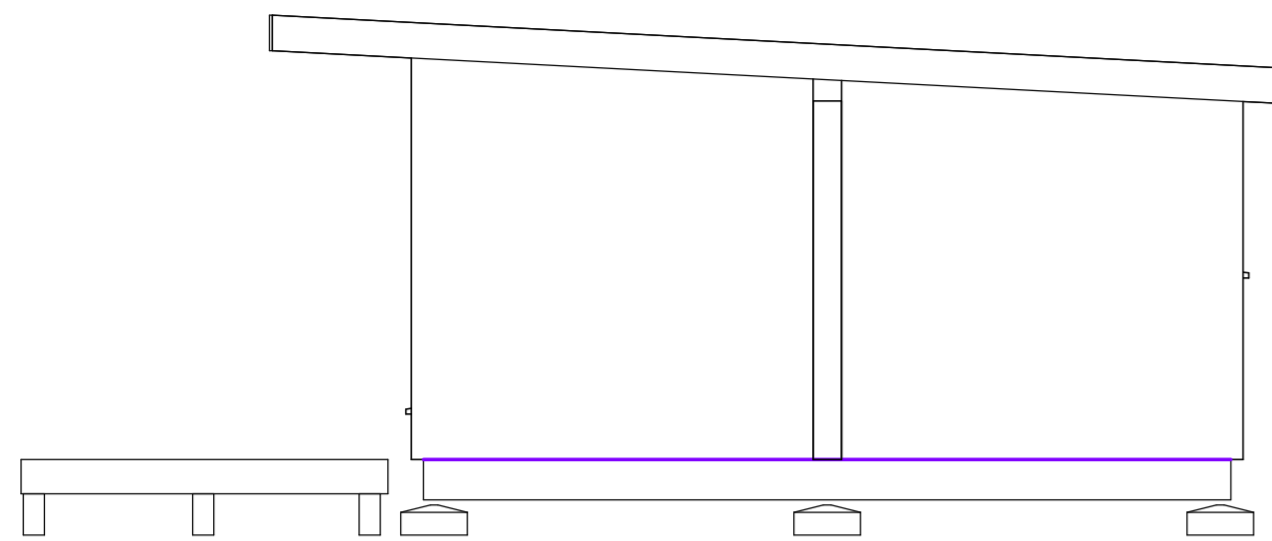
1 East Elevation 1 : 50
