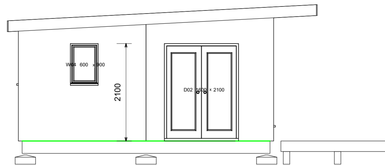
4 West Elevation 1 : 50
