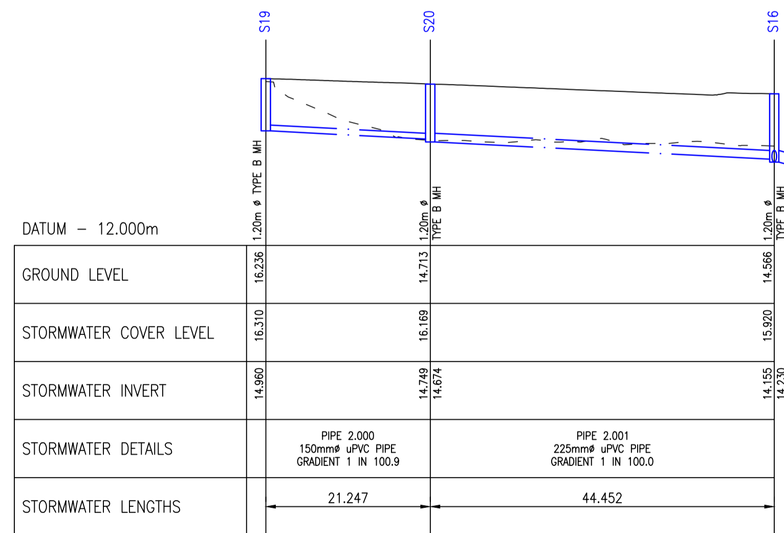
SURFACE WATER SEWER LONG SECTIONS PIPE RUN 2.000 (WEST INLET) (SCALE: Horizontal 1:500, Vertical 1:100)
