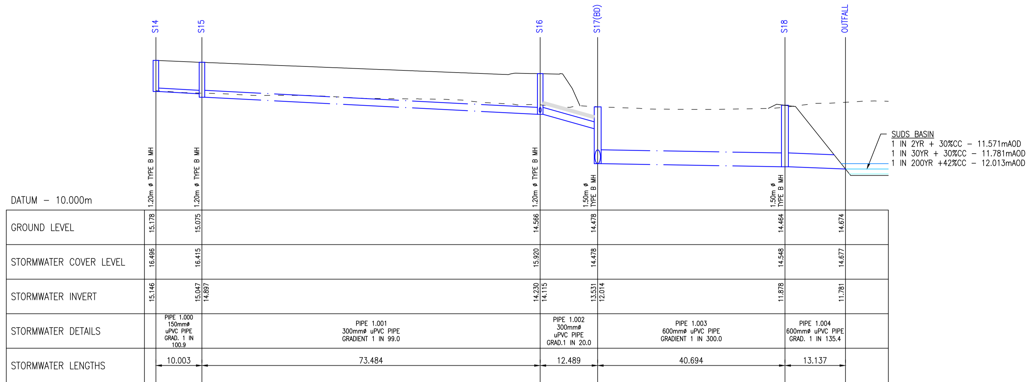
SURFACE WATER SEWER LONG SECTIONS PIPE RUN 1.000 (WEST INLET) (SCALE: Horizontal 1:500, Vertical 1:100)
