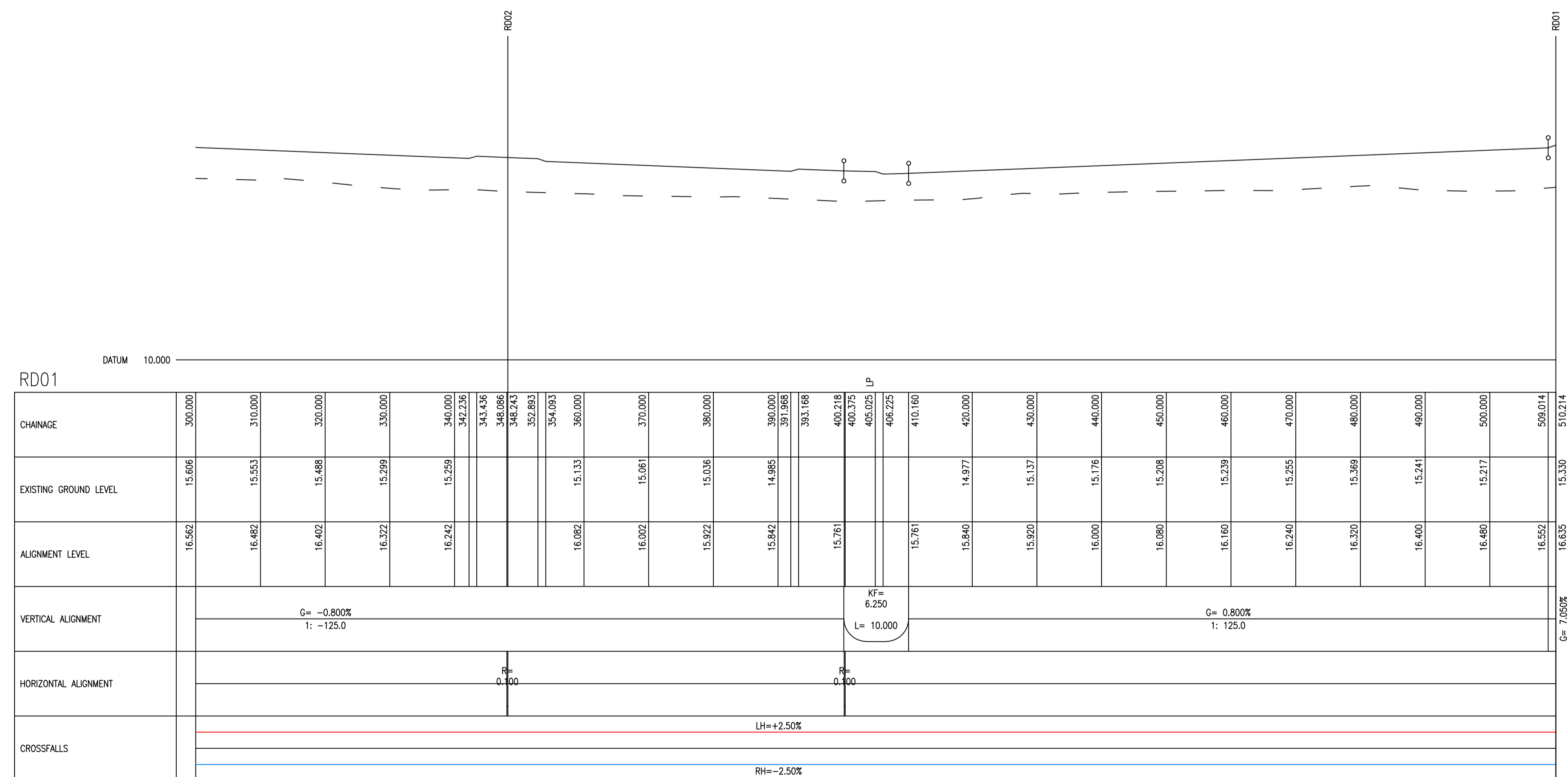
ROAD LONGITUDINAL SECTION THROUGH RD01 CENTRELINE (CH300.000 - 510.214m)
