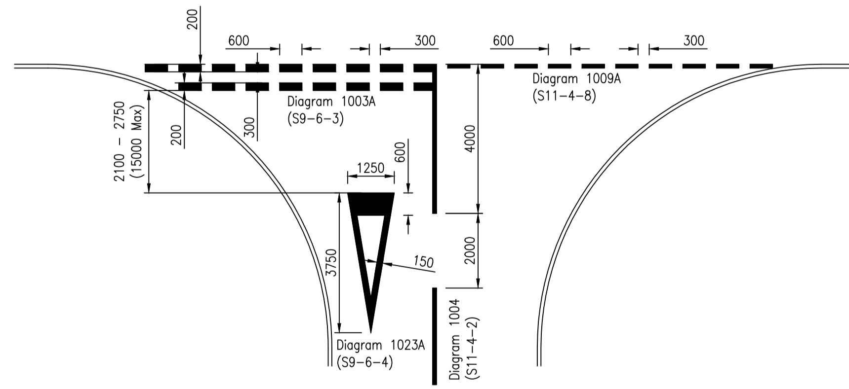
Typical Give Way Junction Detail Scale 1:100
