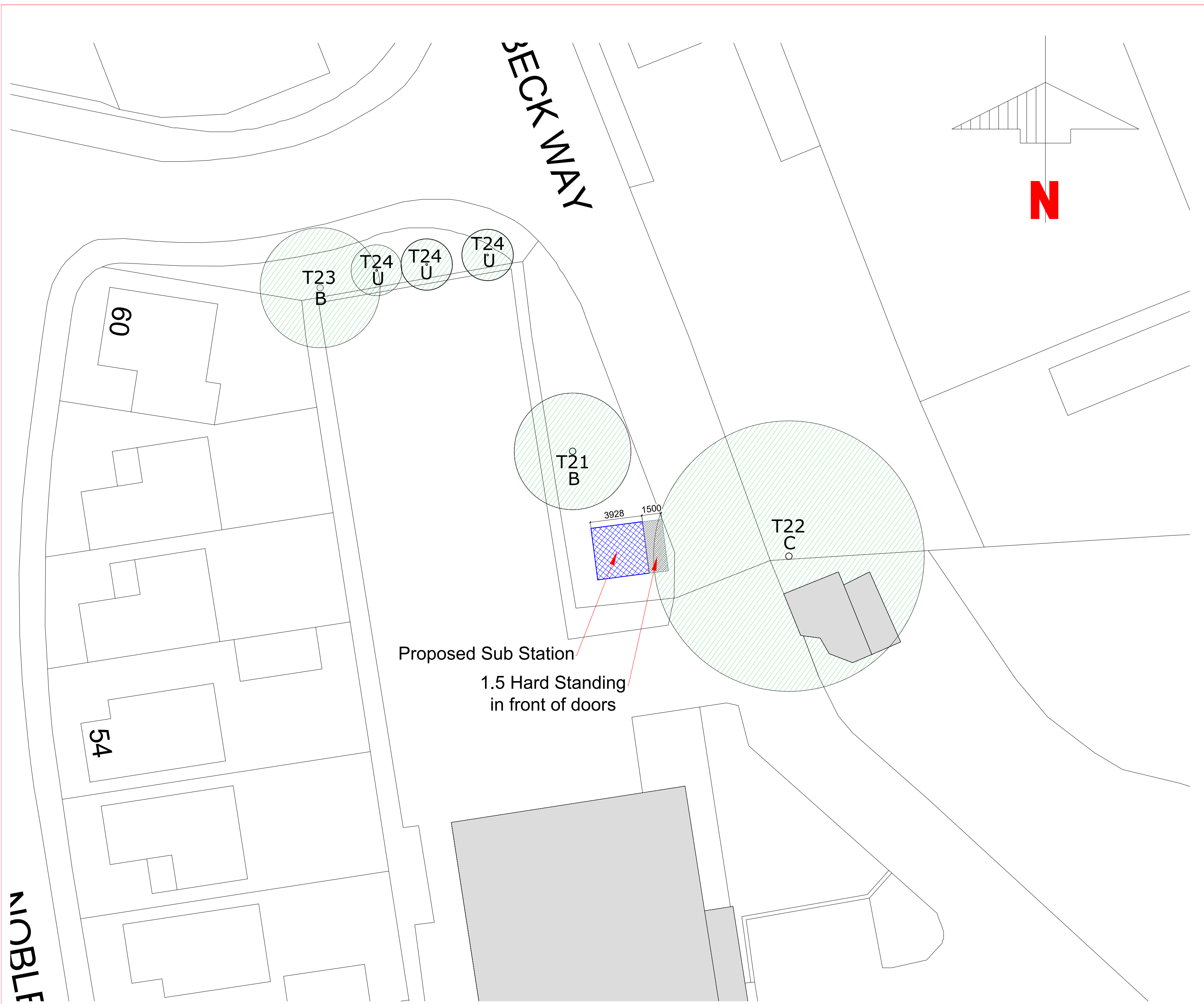
Proposed Sub Station Location - Tree Protection Areas Scale 1:200
