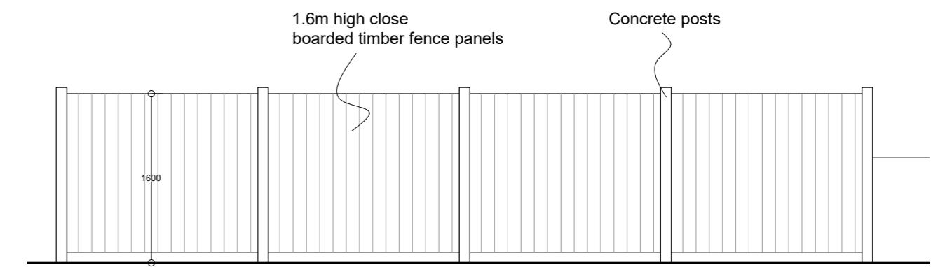
Fence Elevation from Rochester Drive (1:50)
