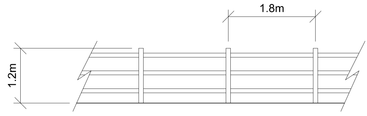
TYPICAL POST AND RAIL FENCE DETAIL
