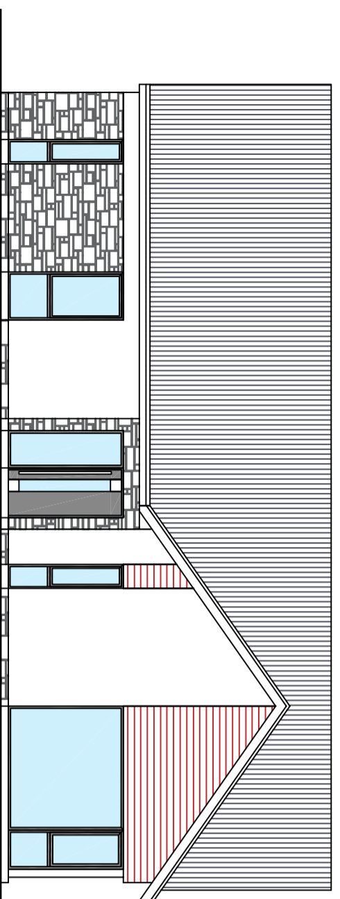
FRONT ELEVATION
