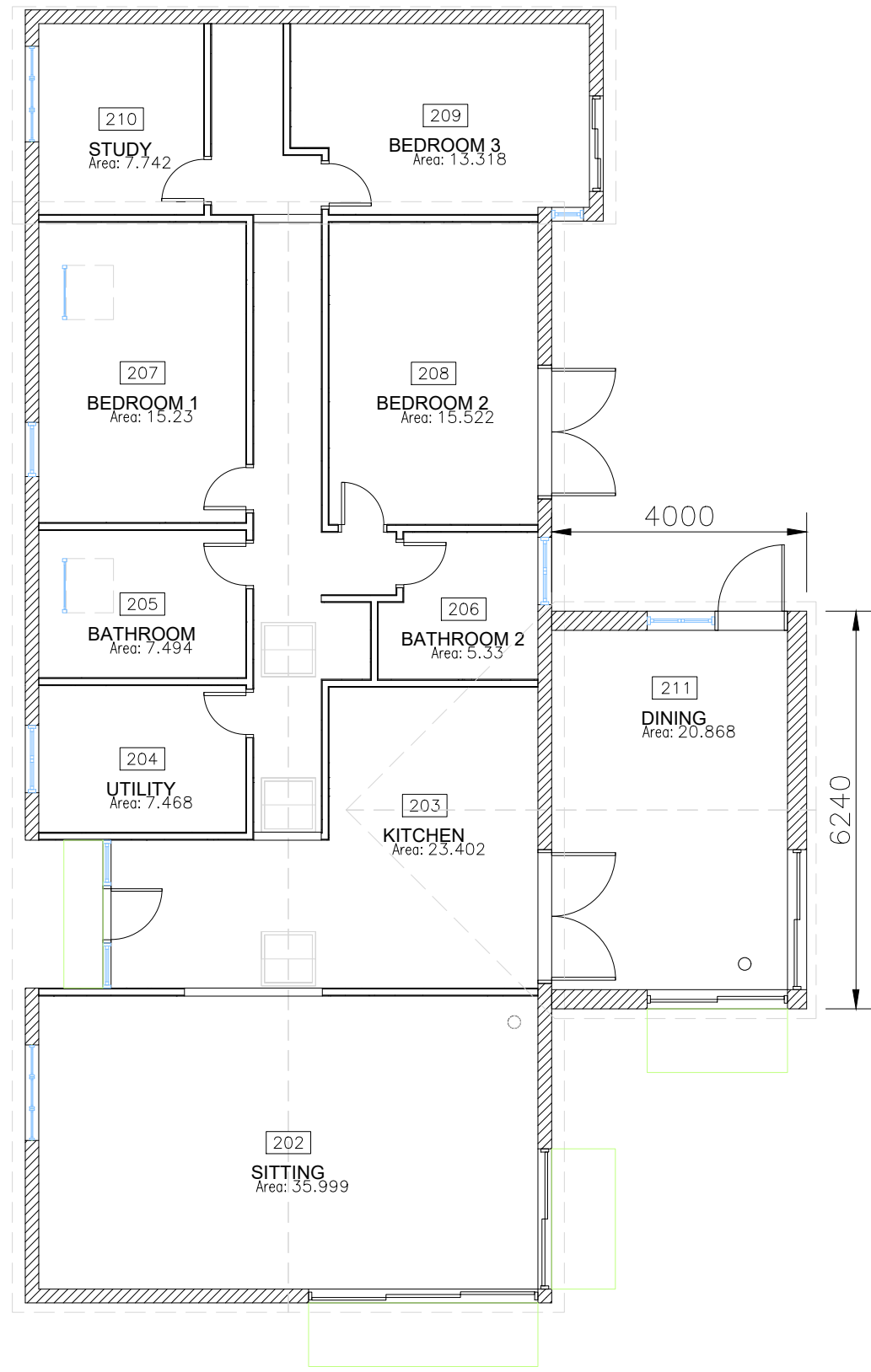
Proposed Floor Plan 1:100
