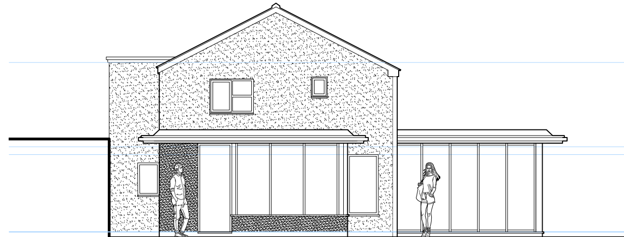
West Elevation
