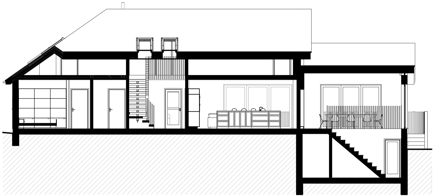
1 Section 1:100
