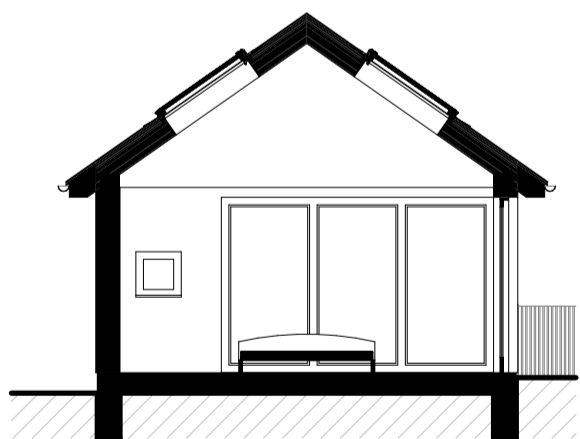
3 Section 1:100
