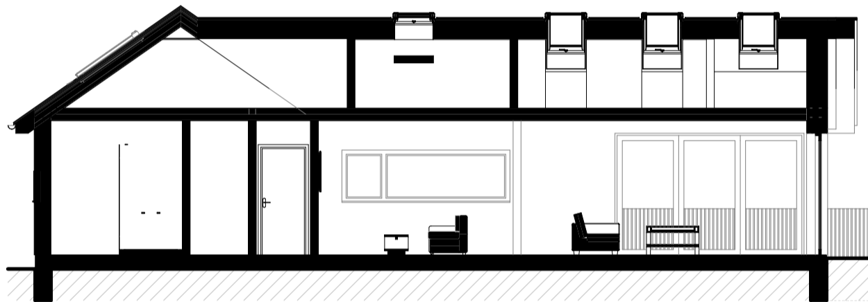
2 Section 1:100
