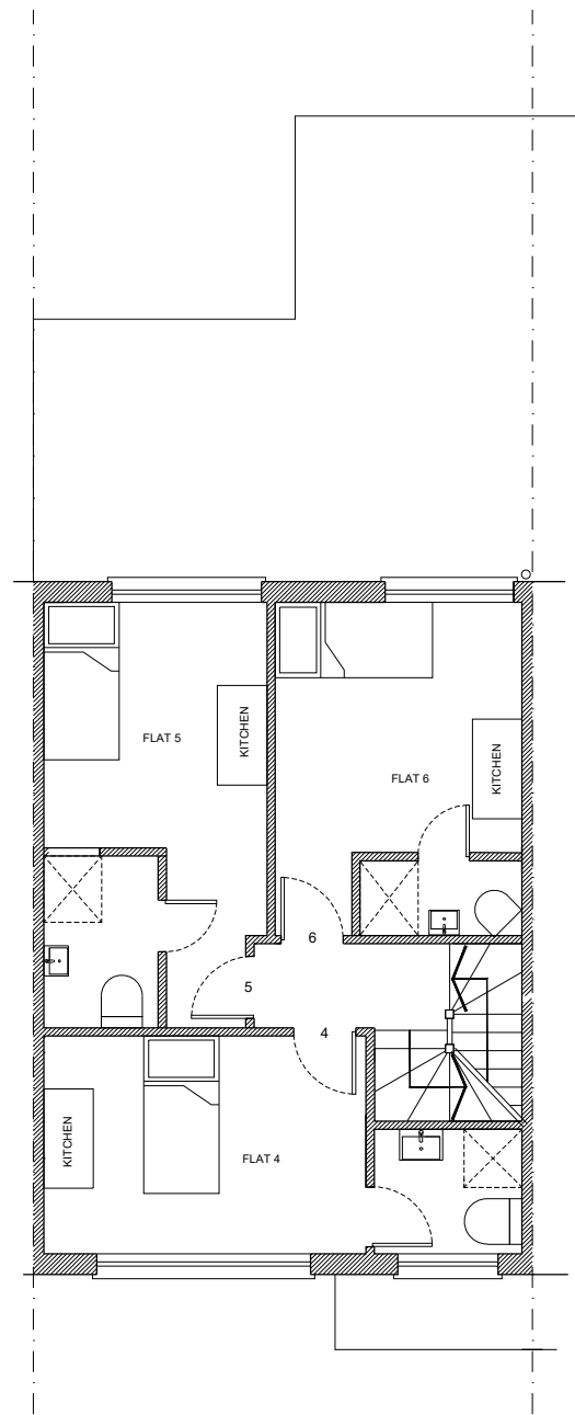
2 EXISTING FIRST FLOOR PLAN SCALE@A1 1:50 SCALE@A3 1:100 PL-001
