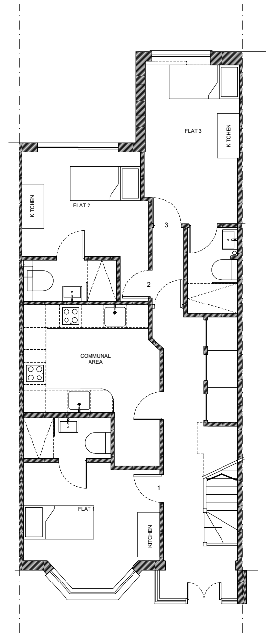
1 EXISTING GROUND FLOOR PLAN SCALE@A1 1:50 SCALE@A3 1:100 PL-001
