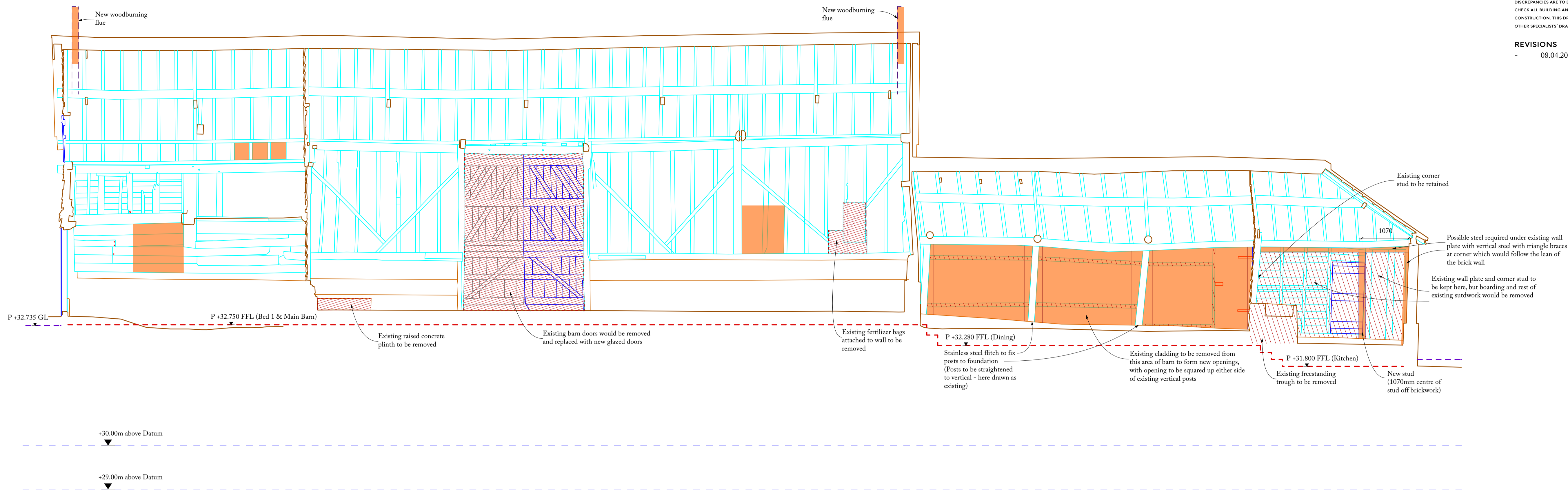
3 MAIN BARN: SECTION 3 as Existing 1:50
