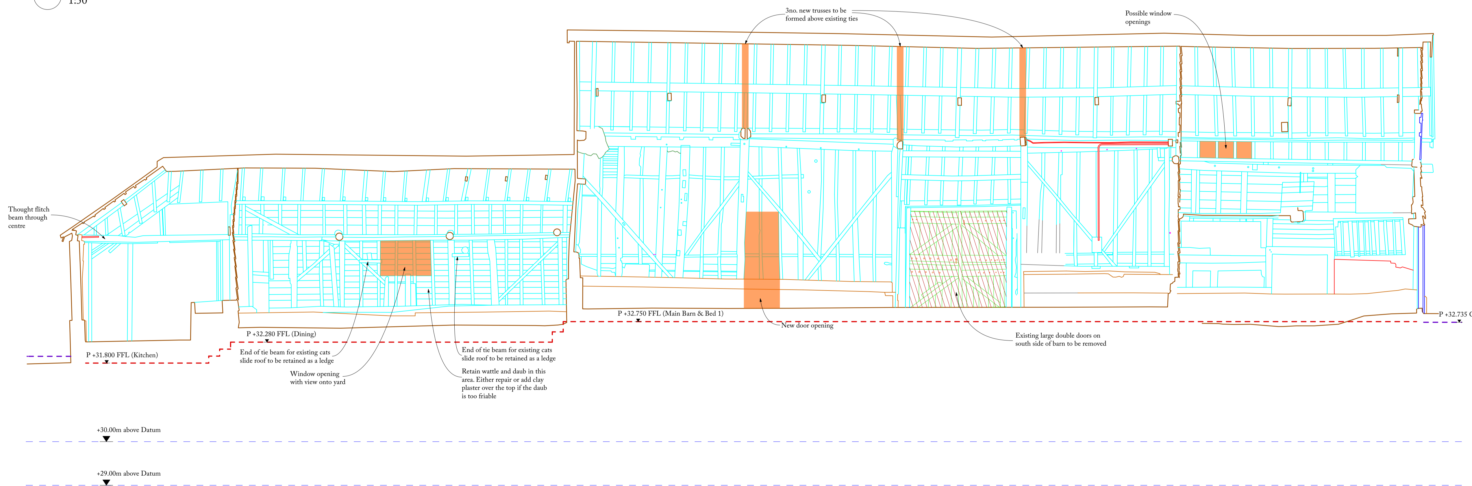
3 MAIN BARN: SECTION 3 as Existing 1:50
