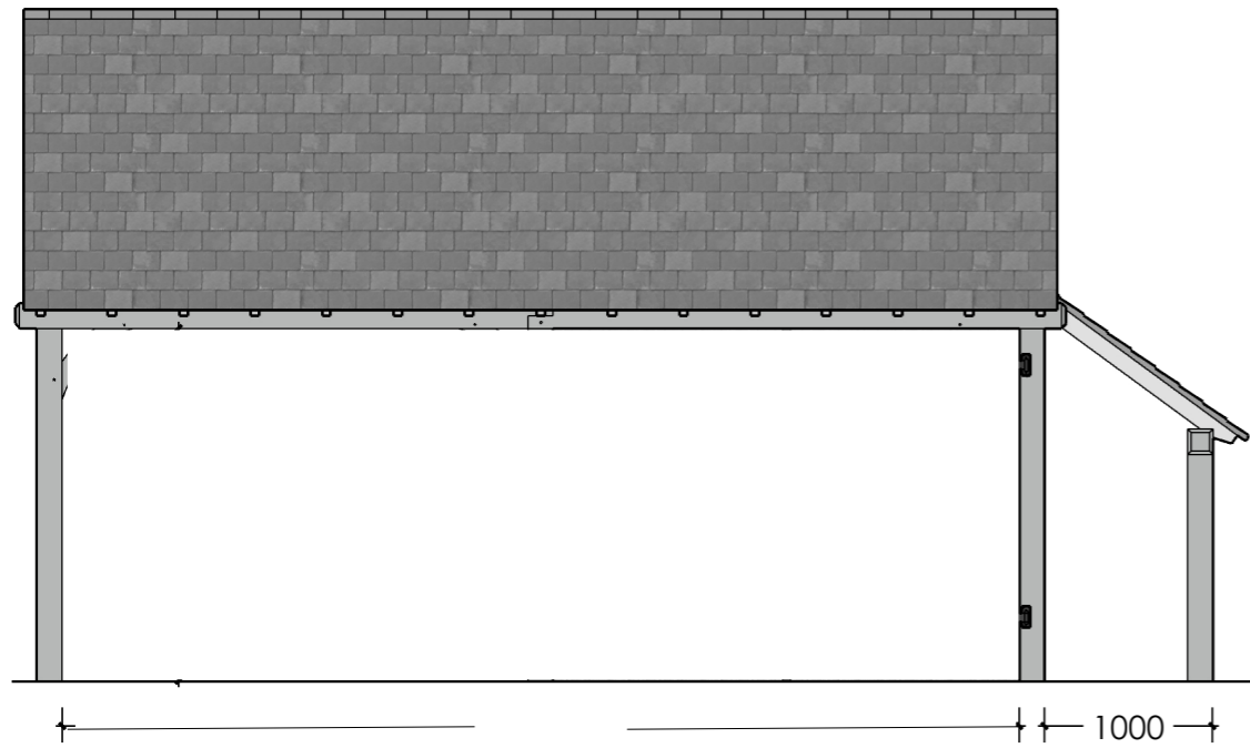
6000 FRONT ELEVATION
