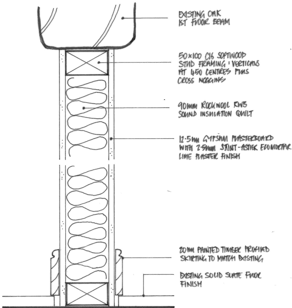
Internal Partition: Vertical Section 1:5 at A4
