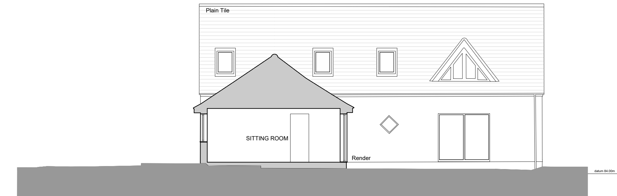
Section AA 1:100
