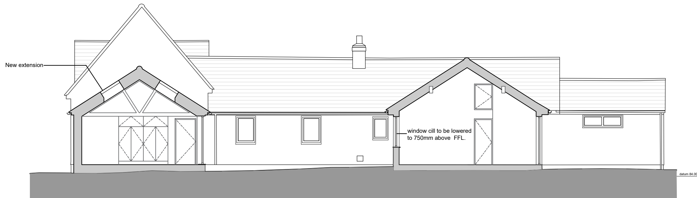
Section CC 1:100
