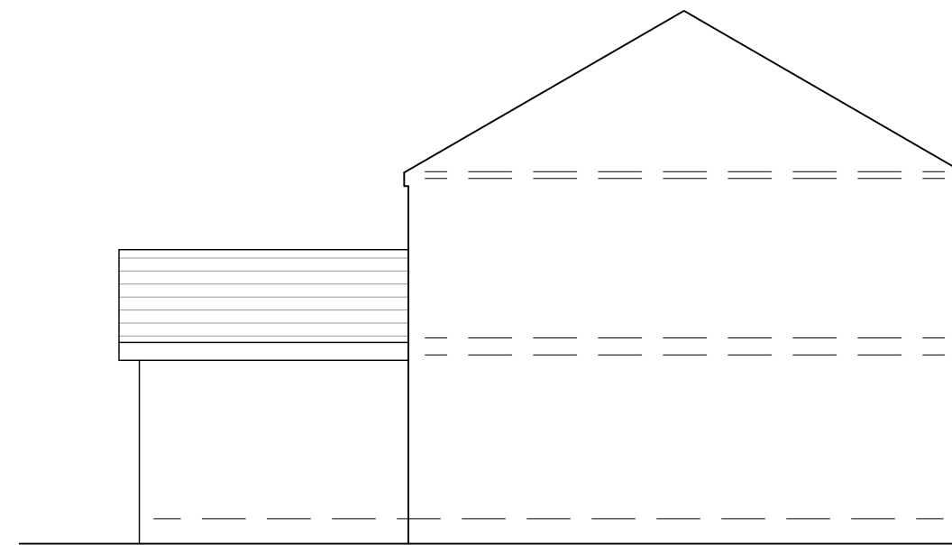
Proposed Side Elevation (no change) 1:100
