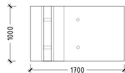
RETAINING WALL PRECAST UNIT PLAN
