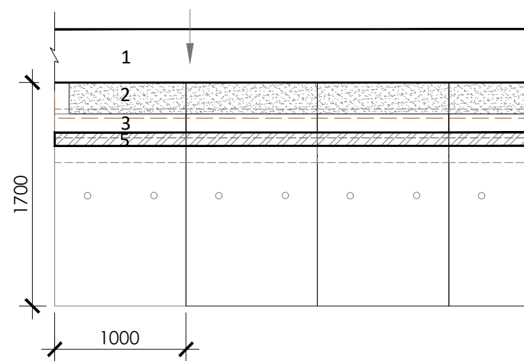
PROPOSED RETAINING WALL DETAIL PLAN 1:20
