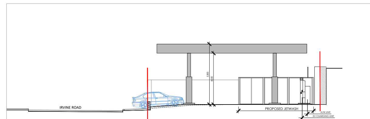
PROPOSED EAST CONTEXTUAL ELEVATION TOWARDS JW/AW/VAC UNITS
