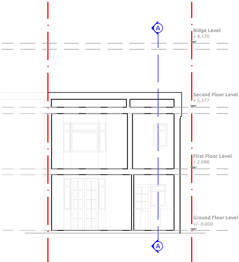
Section B-B
